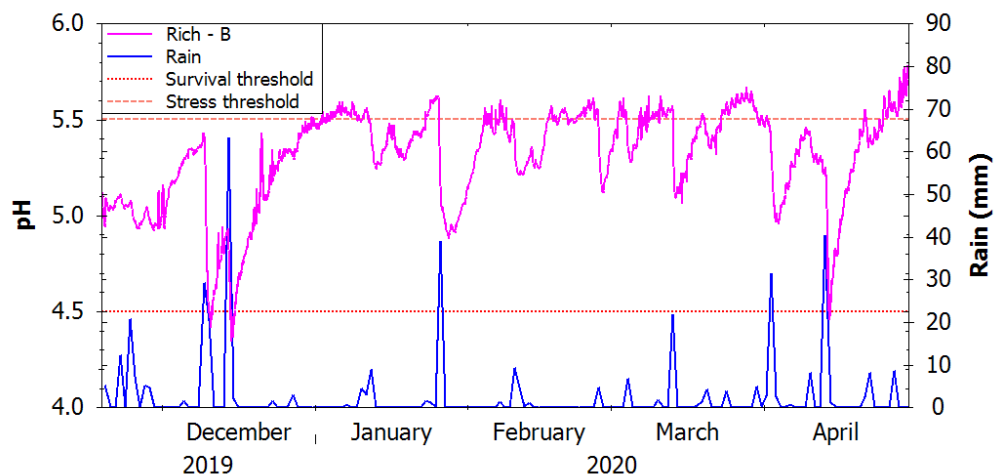
Figure 4. Winter 2019-2020 pH at the downstream Richardson Brook site, within the shell application reach. Stress threshold from Stanley and Trial 1995 and Haines et al. 1990. Survival threshold from Potter 1982. Rainfall data from Weather Underground.
