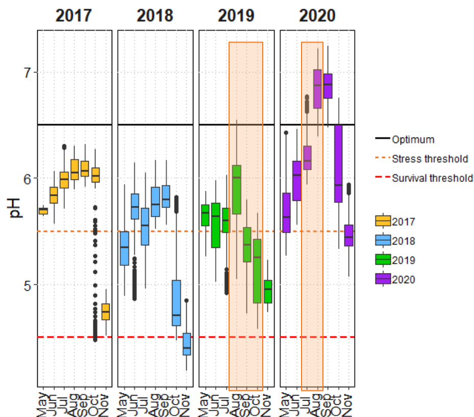
Figure 6. Monthly pH at the downstream Richardson Brook site (Rich-B). Each box represents the interquartile range, with the horizontal line representing the median, and whiskers extending to the minimum and maximum values observed, except where values are considered statistical outliers (dots). Optimum pH from Kroglund and Staurnes 1999 and Kroglund et al. 2008. Stress threshold from Stanley and Trial 1995 and Haines et al. 1990. Survival threshold from Potter 1982. Orange boxes represent shell additions in 2019 and 2020.
