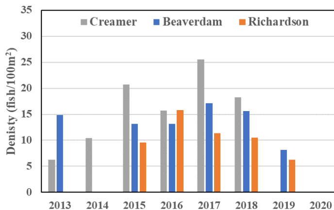
Figure 2. Salmon density in three of the study streams from 2013–2020. High flows prevented data collection in Creamer Brook in 2019. Extremely low flows prevented data collection in 2020. Data from MDMR electrofishing surveys.
