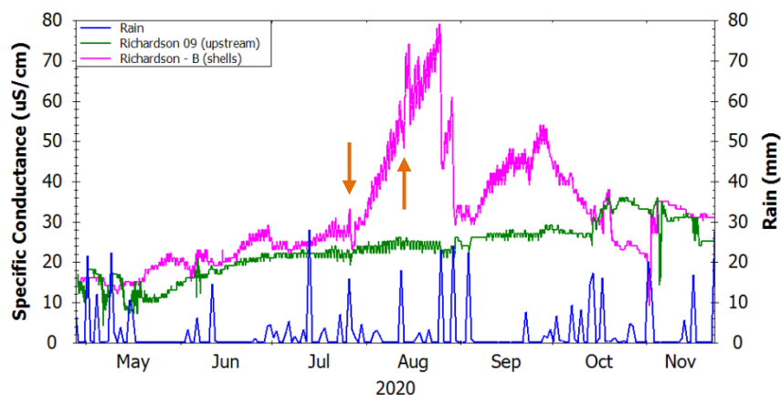
Figure 7. Specific conductance and rainfall at the two Richardson Brook sites in 2020. Orange arrows indicate days on which shells were added at the downstream site. Rainfall data from Weather Underground.
