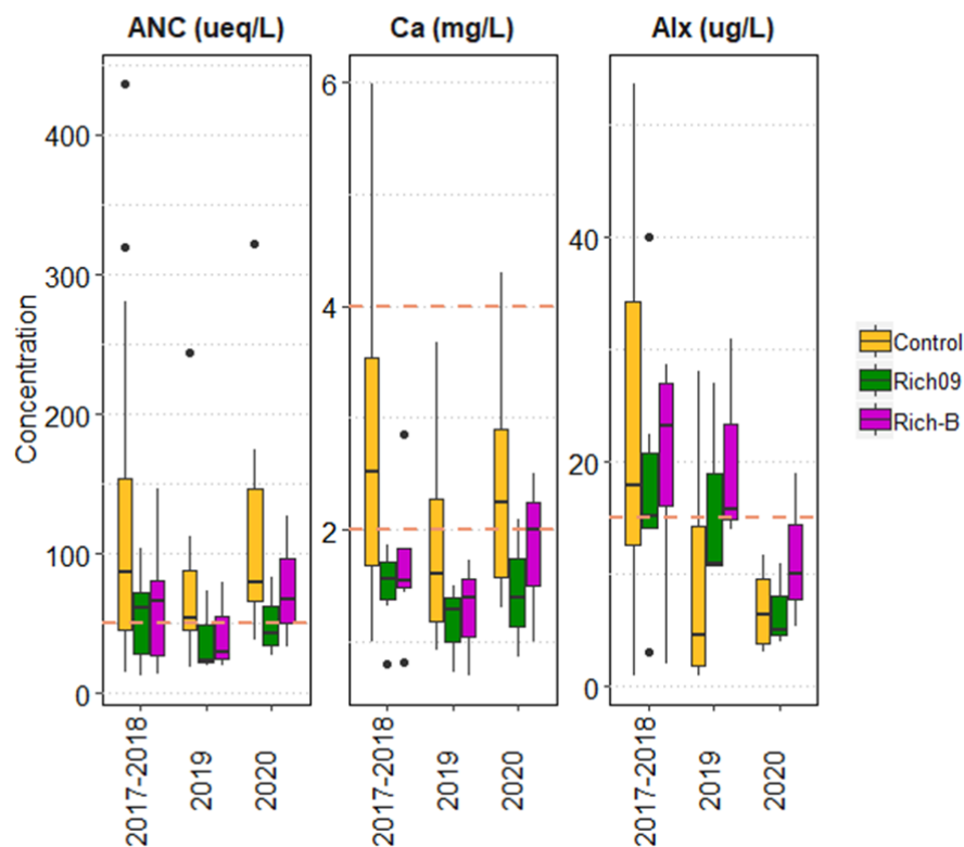
Figure 8. Acid neutralization capacity (ANC), calcium (Ca) and exchangeable aluminum (Alx). 2017-2018 represents baseline conditions. Shells were added to Rich-B in 2019 and 2020. Control includes Creamer and Barney Brooks and Beaverdam Stream. Each box represents the interquartile range, with the horizontal line representing the median, and whiskers extending to the minimum and maximum values observed, except where values are considered statistical outliers (dots). Sample size: control 2017-2018 n = 17; 2019 and 2020 n = 8; Rich09 and Rich-B 2017-2018 n = 6; 2019 and 2020 n = 3. ANC stress threshold of <50 µeq/L from Driscoll et al. 2001. Calcium stress thresholds of <4 mg/L from M. Whiting (pers. comm.) and <2 mg/L from Baker et al. 1990 and Baldigo and Murdoch 2007. Alx stress threshold of >15 µg/L from EIFAC as cited in Dennis and Clair 2012.
