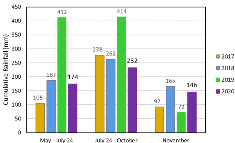
Figure 3. Cumulative annual rainfall. The three time periods represent spring pre-treatment, summer-fall shell treatment, and November post-treatment, based on shell applications in 2019-2020. Data from Weather Underground stations KMEALEXA2, KMEBAILE9 and KMEPRINC2.
