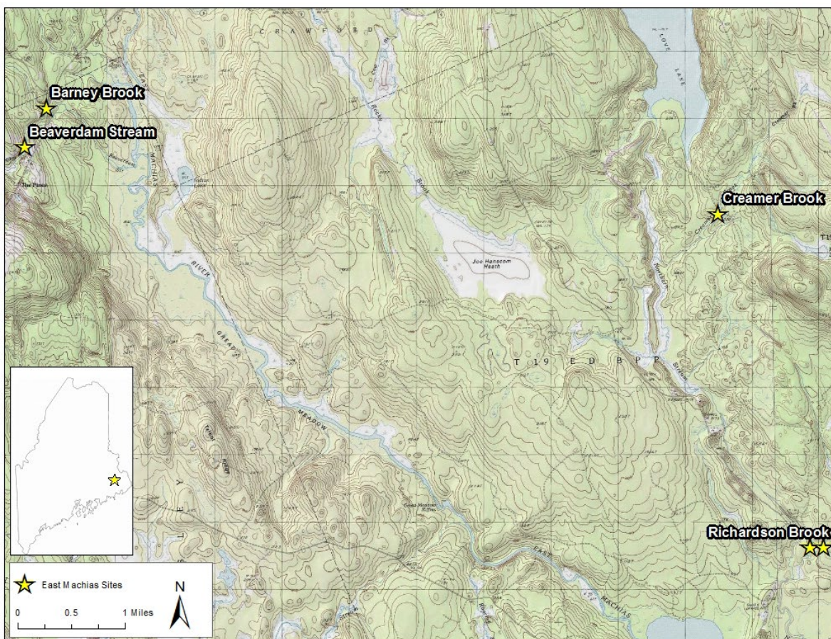
Figure 1. Map of the five study sites on four tributaries to the East Machias River. On Richardson Brook, samples were collected below the road crossing and above the shell treatment reach.
